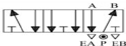
5/3 Valve
