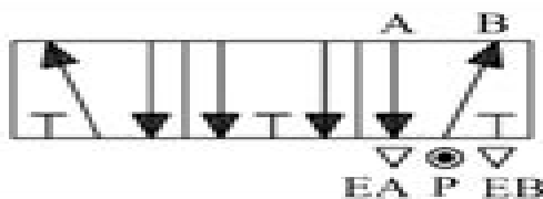
5/3 Valve
