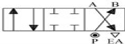
4/3 Valve
