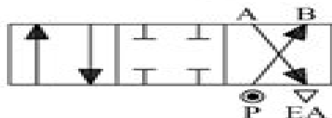
4/3 Valve
